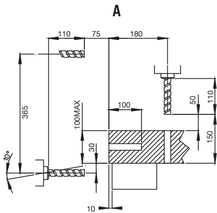
Fresa standard Fraise standard Standard milling unit Cabezal fresador standard
