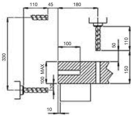
Fresa standard Fraise standard Standard milling unit Grupo fresa standard
